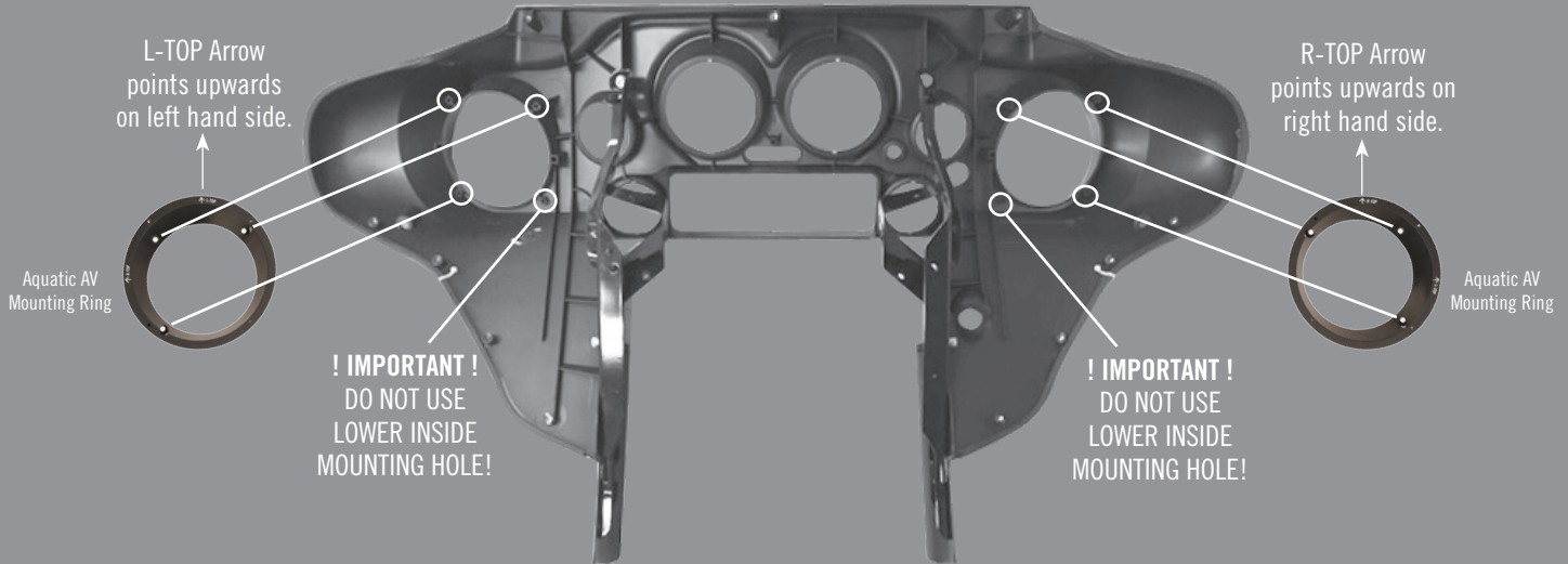
Harley-Davidson Batwing Fairing
